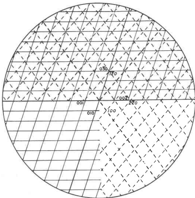
FIG. 6. 0kl reciprocal lattice plane of rosenhahnite in solid lines, vertical indices. hko reciprocal lattice plane of triclinic wollastonite in dashed lines, slanting indices. Scale matches Figure 5. The overlap of lattices in upper part of drawing corresponds to the dual pattern reproduced in Figure 5.
