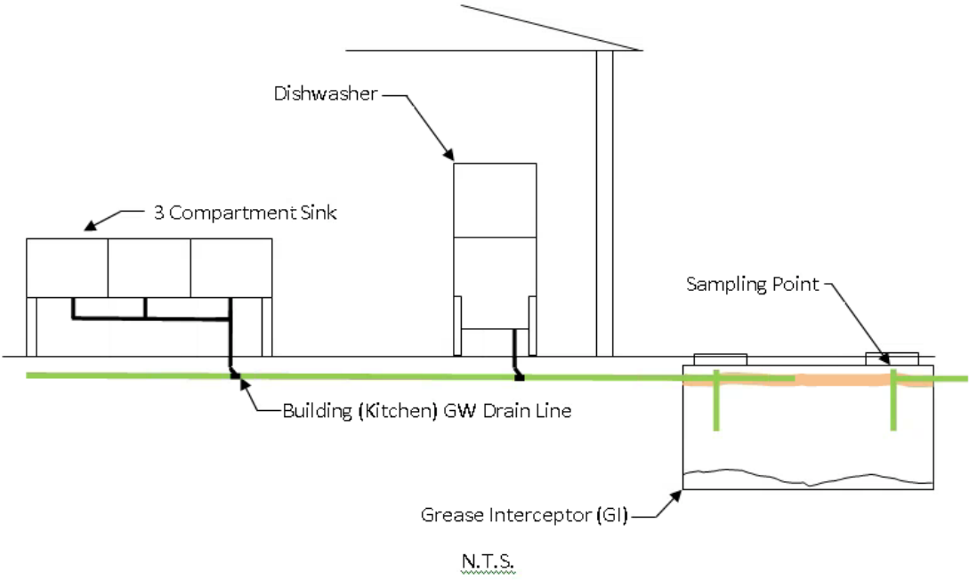
Figure 2. Grease Interceptor and Sampling Point Adequate Location
