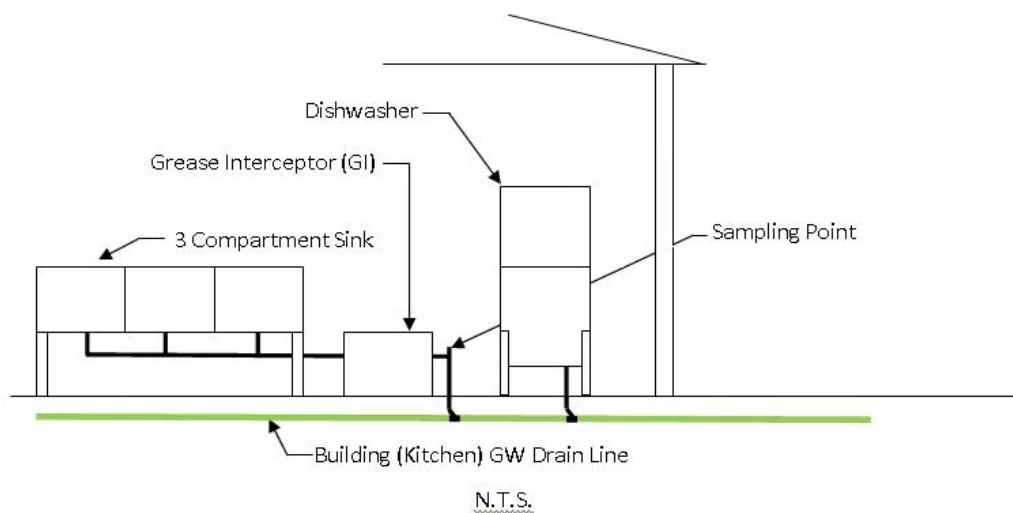
Figure 1. Grease Interceptor Location Inadequate
