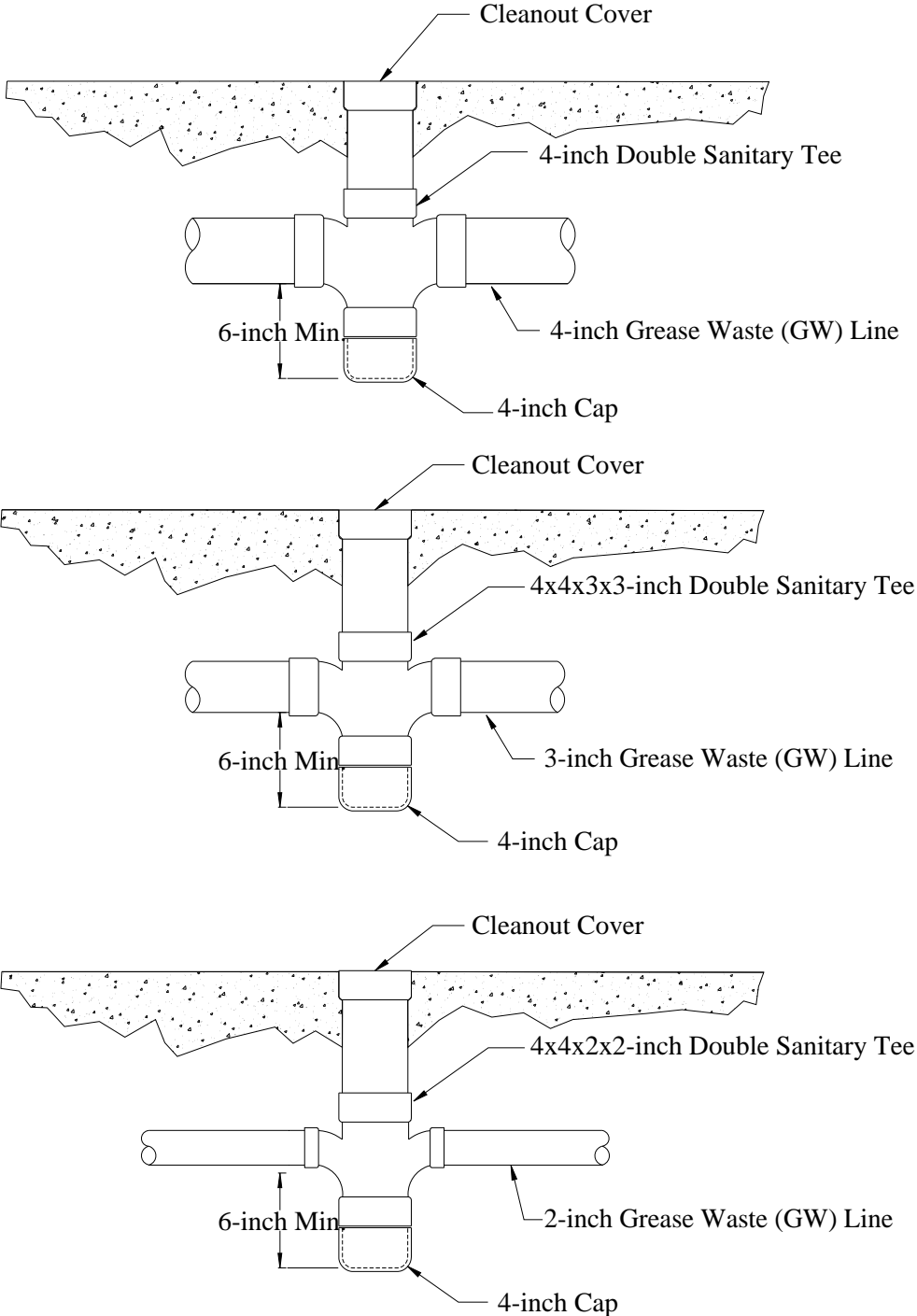
Figure 6: Sampling Point Schematics (NTS)
