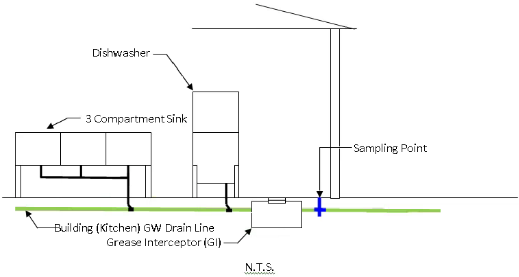
Figure 3. Grease Interceptor adequate Location
