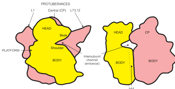
FIGURE 2. Contours of two ribosomal subunits, the small 30 S (yellow) and the large 50 S (red), associated in the full 70 S ribosome, with designations of some morphological features. Left , the so-called overlap projection when the 30 S subunit is facing the viewer and covers part of the 50 S subunit; right , the lateral projection viewed from the side of the L7/L12 stalk. CP, central protuberance.
