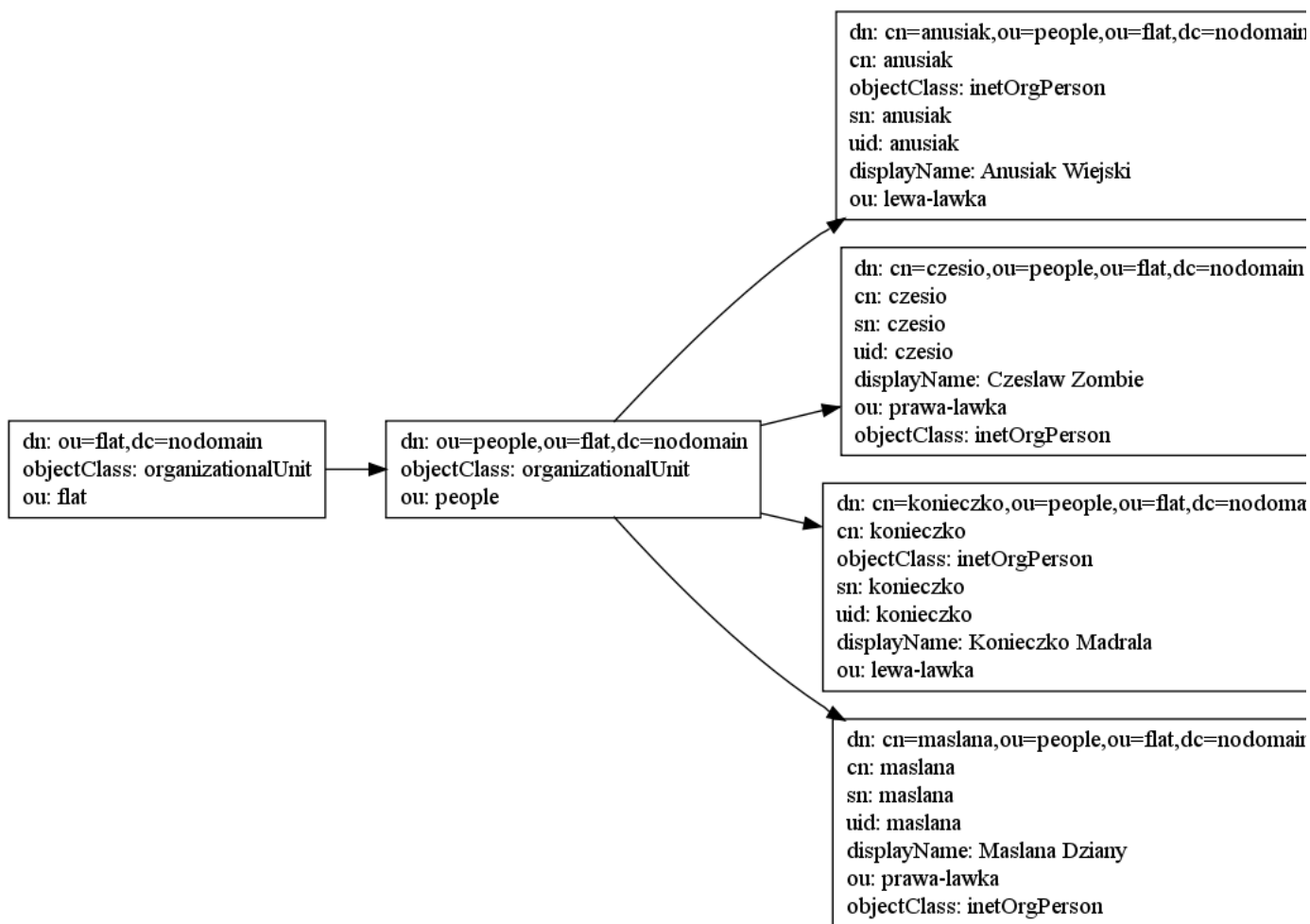
Figure 3.1: Flat DIT graph
