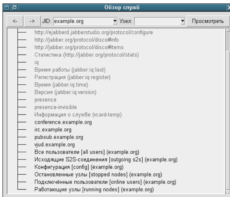
Figure A.1: Service Discovery when xml:lang='ru'
