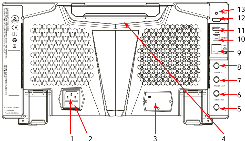
Figure 1-8 Rear Panel
