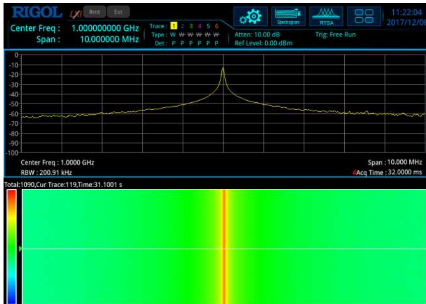
Figure 3-4 Spectrogram View
