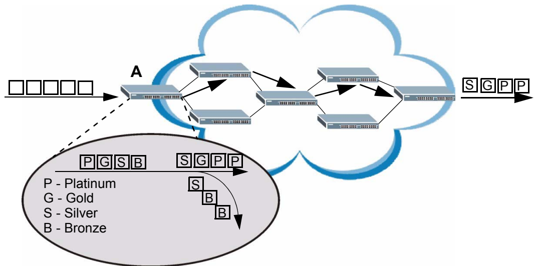
Figure 138 DiffServ Network
