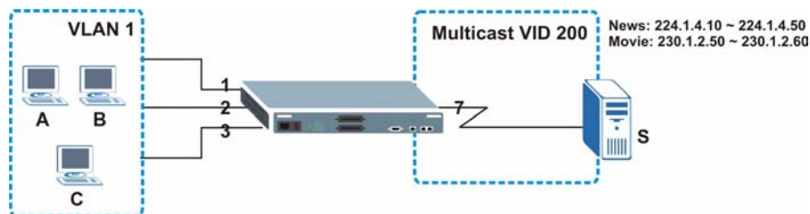
Figure 104 MVR Configuration Example
