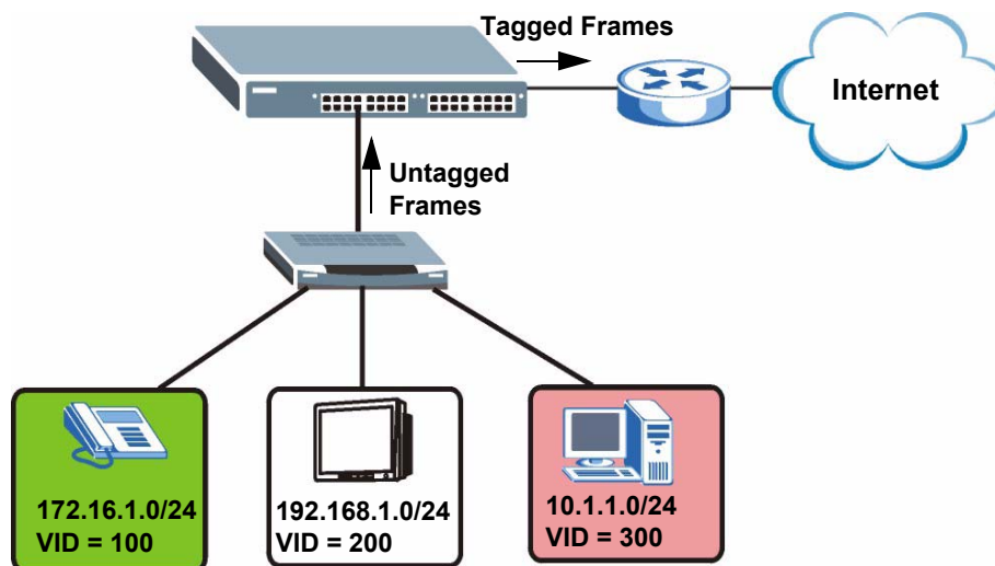
Figure 51 Subnet Based VLAN Application Example
