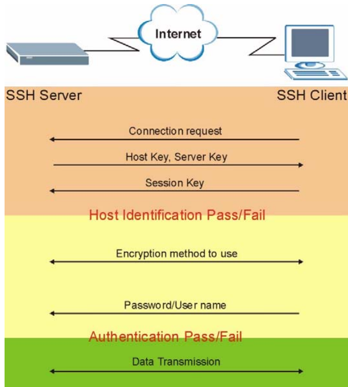
Figure 160 How SSH Works
