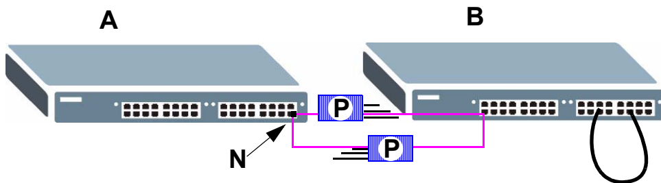
Figure 129 Loop Guard - Probe Packet
