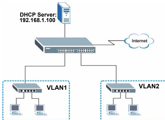
Figure 143 Global DHCP Relay Network Example
