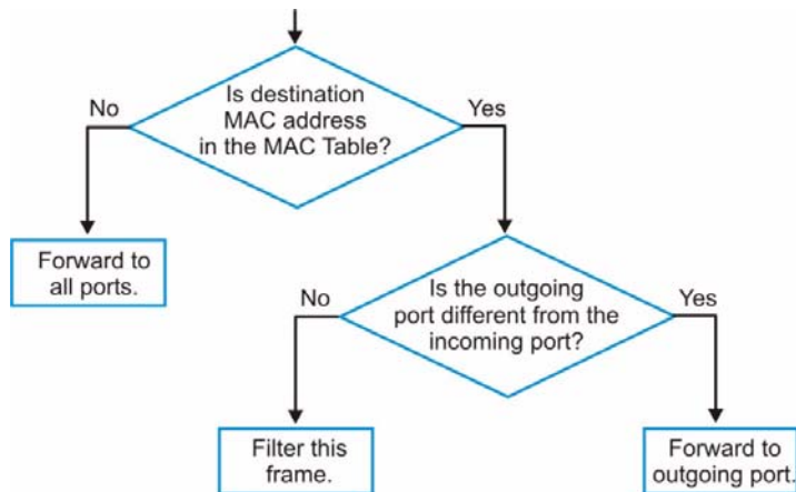
Figure 176 MAC Table Flowchart
