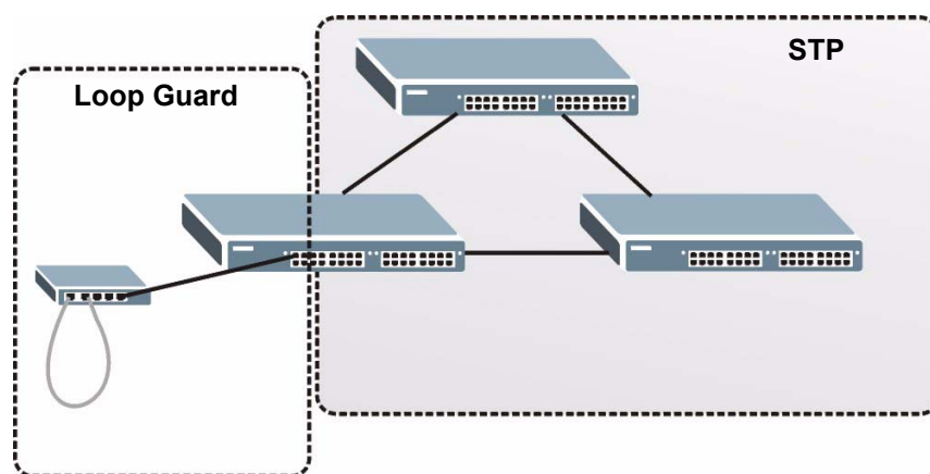
Figure 127 Loop Guard vs. STP
