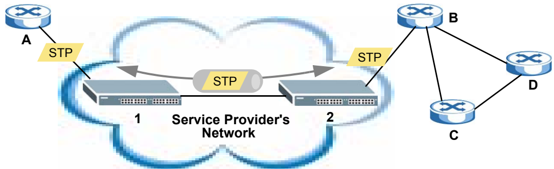
Figure 133 L2PT Network Example
