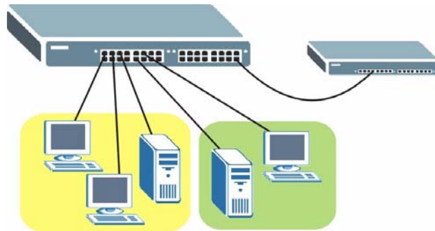
Figure 53 Protocol Based VLAN Application Example
