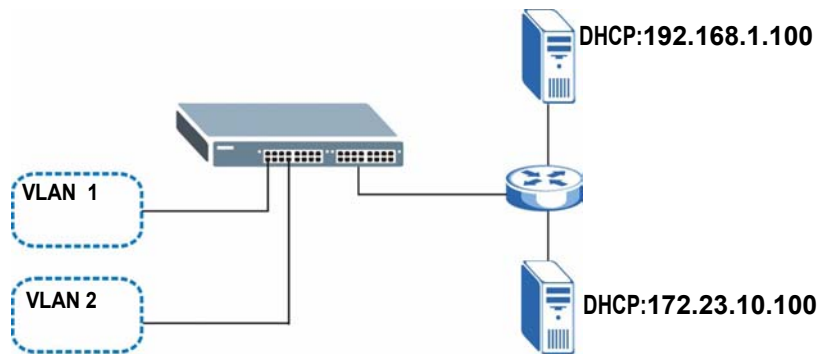
Figure 146 DHCP Relay for Two VLANs
