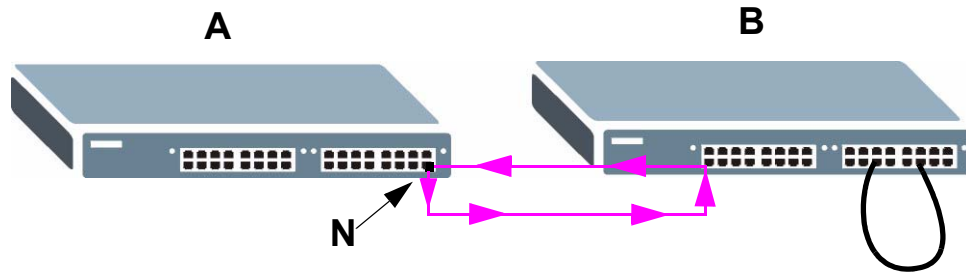
Figure 128 Switch in Loop State
