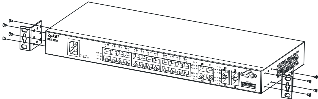
Figure 7 Using a #2 Philips screwdriver, install the M3 flat head screws through the mounting bracket holes into the Switch.
