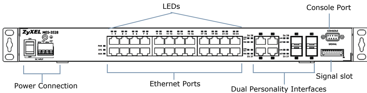
Figure 10 Front Panel (DC)
