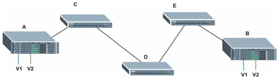
Figure 45 Port VLAN Trunking
