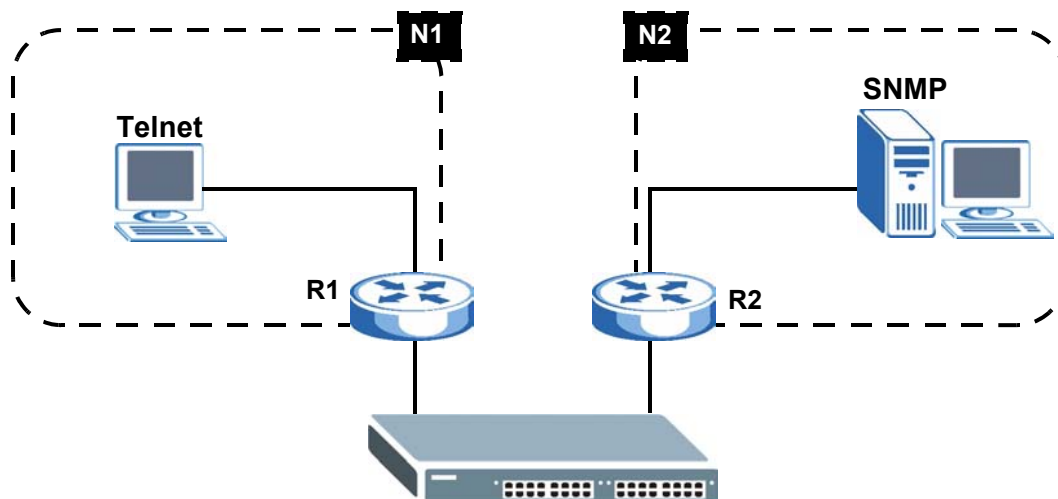
Figure 135 Static Routing Overview
