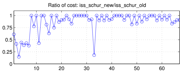
FIG. 6.3. Experiment 2: ratios of the cost of iss_schur_new divided by the cost of iss_schur_old .
