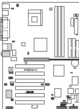
P4B533-V Accelerated Graphics Port (AGP)
