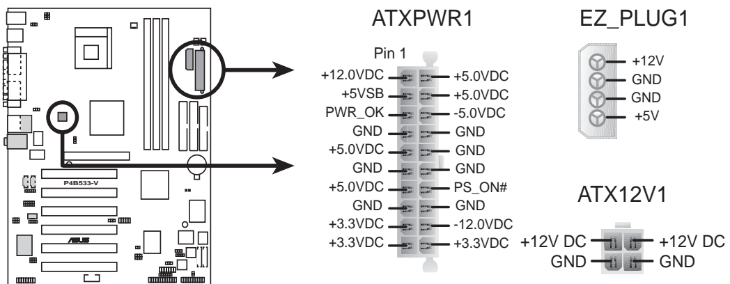
P4B533-V ATX & Auxiliary Power Connectors
