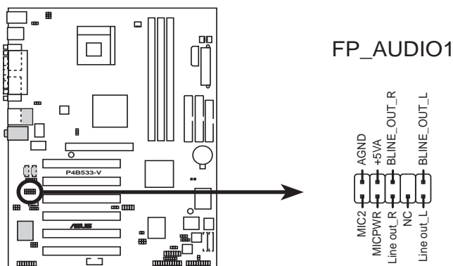
P4B533-V Front Panel Audio Connector
