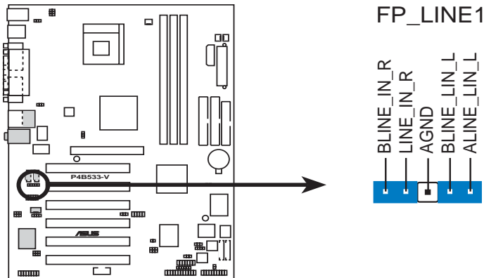
P4B533-V LINE_IN Connector
