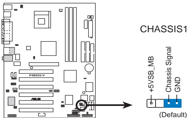
P4B533-V Chassis Alarm Lead
