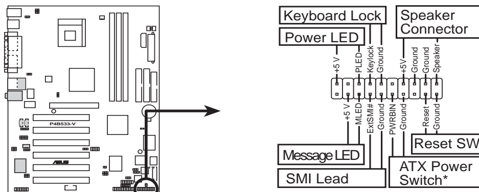
P4B533-V System Panel Connectors
