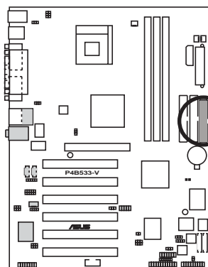
P4B533-V Floppy Disk Drive Connector
