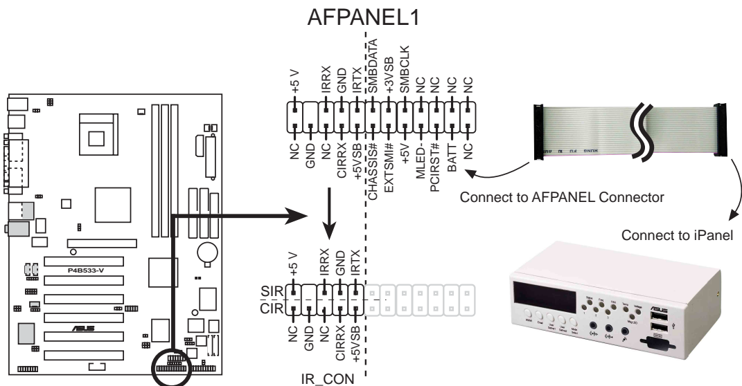
P4B533-V iPanel Connector
