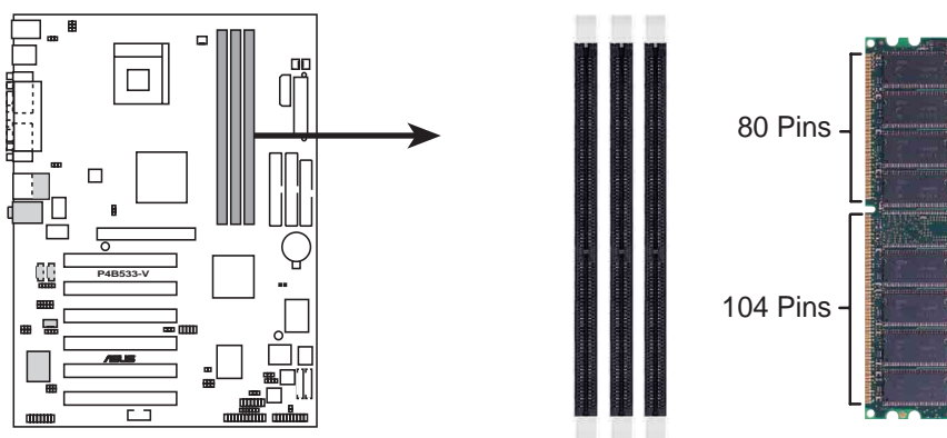
P4B533-V 184-Pin DDR DIMM Sockets
