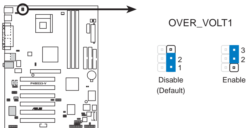
P4B533-V OVER_VOLT Setting
