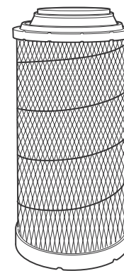
Radial seal HD air filter w/ urethane end caps - bottom end has raised sealing area - top end has "dump hole"
