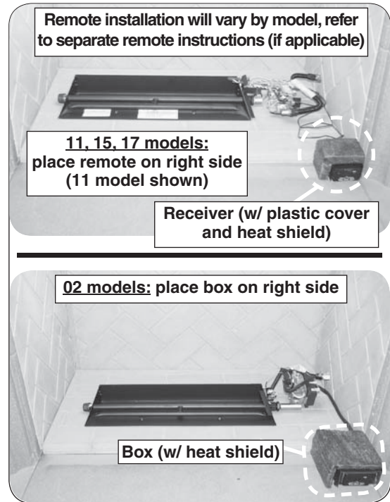
Fig. 18-1 Install remote receiver and heat shield (as applicable)
