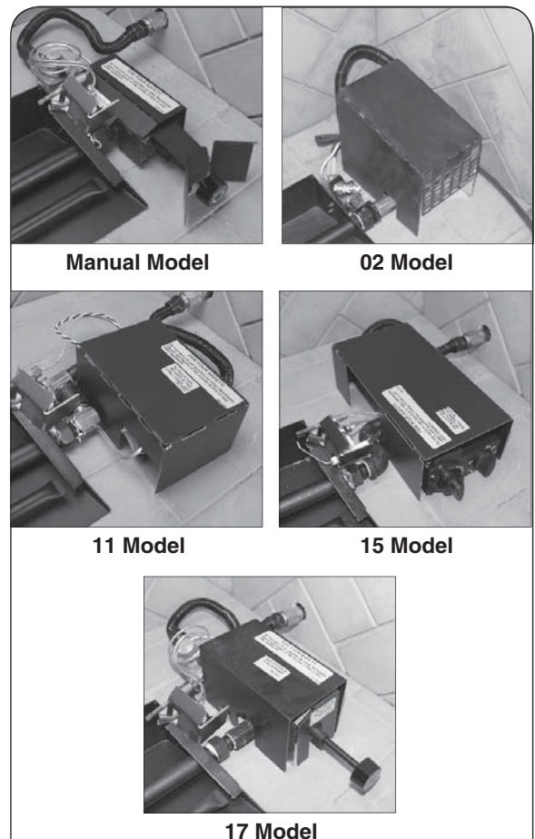
Fig. 18-1 Install remote receiver and heat shield (as applicable)
