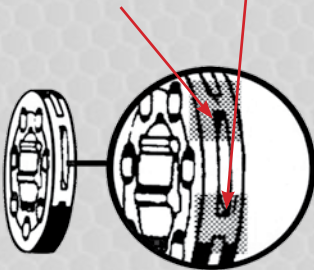
Concave marks worn into rim sprocket teeth
