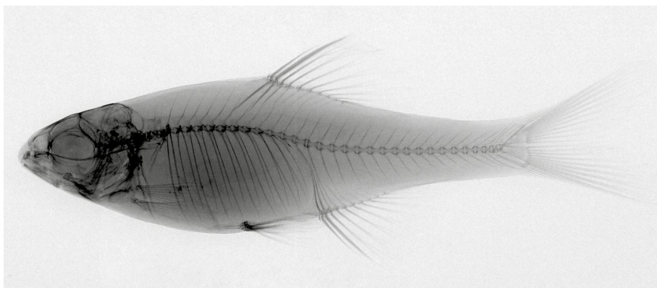
Fig. 11. Radiograph of Rhodeus nigrodorsalis sp. nov. (SOU 1712001, holotype, ♂, 37.0 mm SL).
