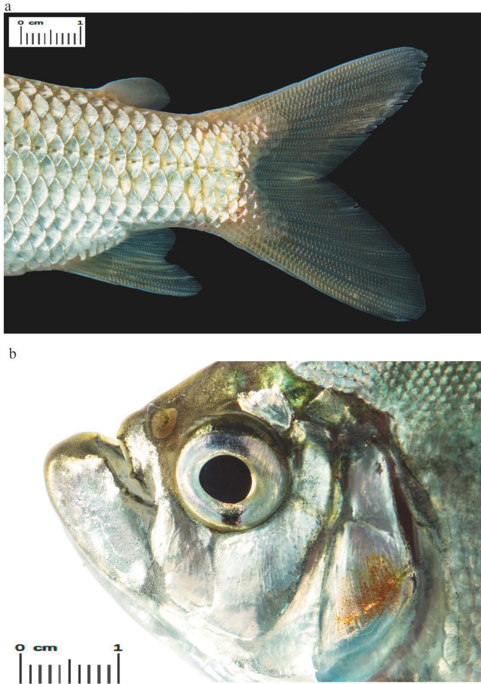
FIGURE 12. Detailed images of the lateral line in a. Cyphocharax magdalenae (Characiformes: Curimatidae) and b. bones of the head in Catoprion mento (Characiformes: Serrasalminidae).
