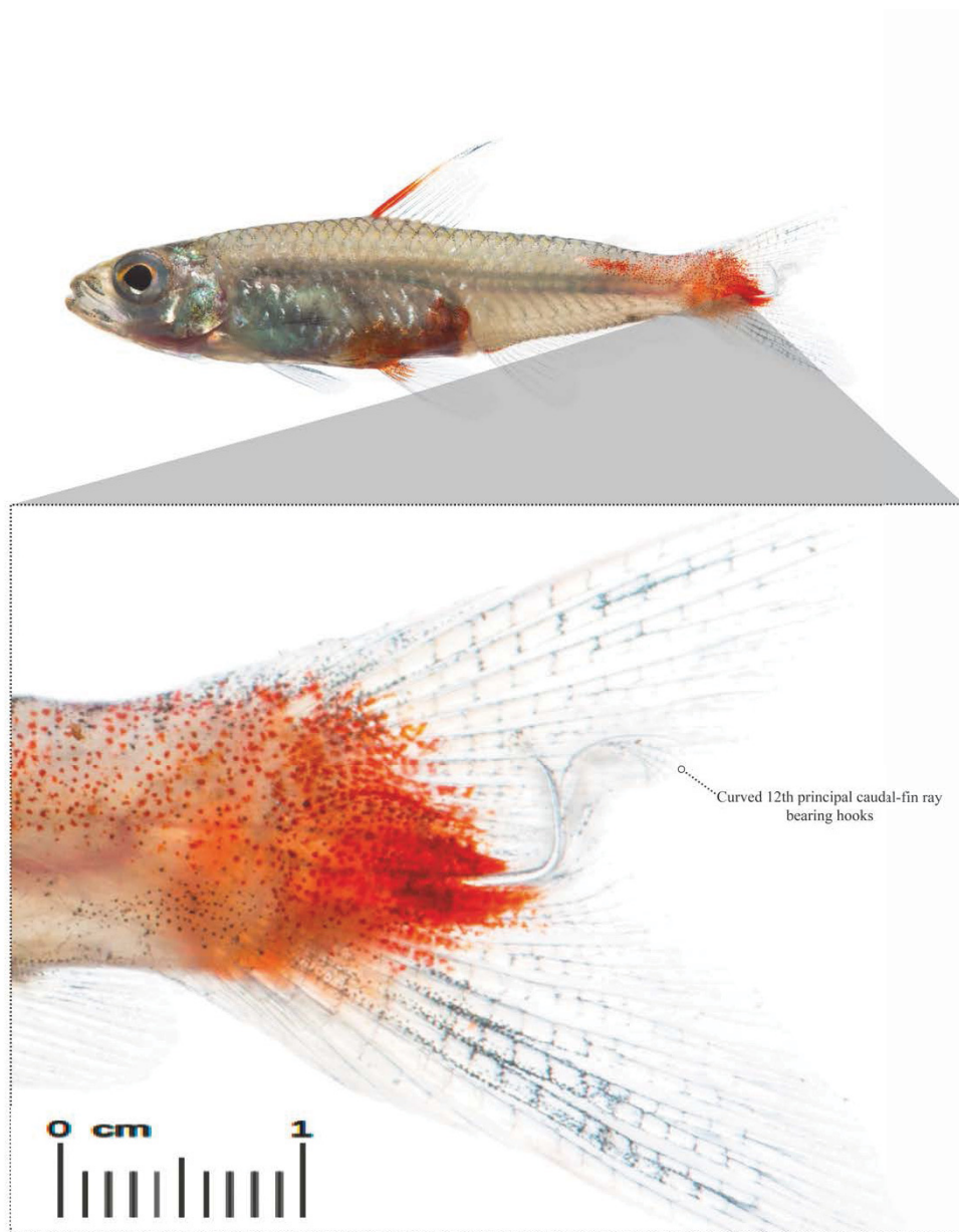
FIGURE 10. Photos highlighting diagnostic character of miniature characid Brittanichthys (Characiformes: Characidae). Mature male has a unique type of caudal fin with the 12th principal caudal-fin ray thickened, elongate, sigmoidally-curved, and projecting slightly to one side.
