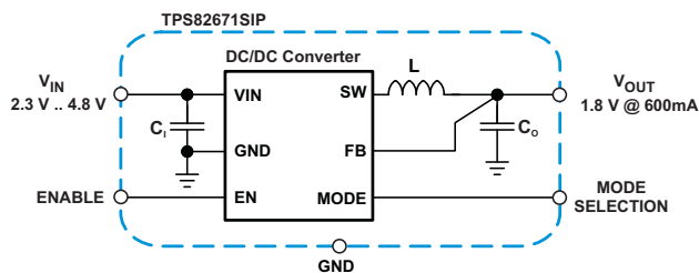
Figure 1. Typical Application
