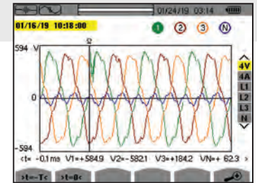
TRANSIENT MODE
