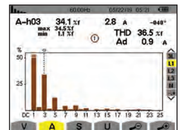
HARMONICS MODE
