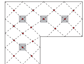
Measure and record multiple measurements to create an illuminance map of the room or area of interest
