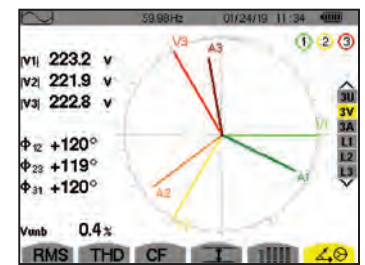
PHASOR DIAGRAM
