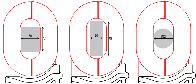
CLAMPING CHARACTERISTICS
