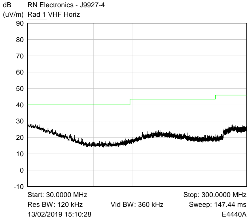
Plot of Peak emissions for VHF Horizontal against the QP limit line.
