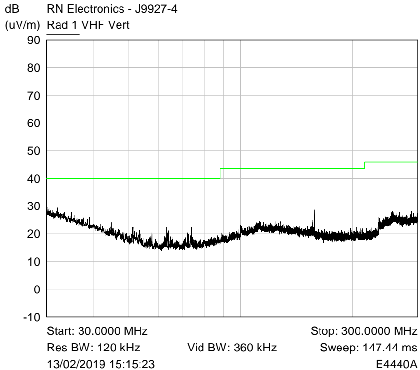
Plot of Peak emissions for VHF Vertical against the QP limit line.
