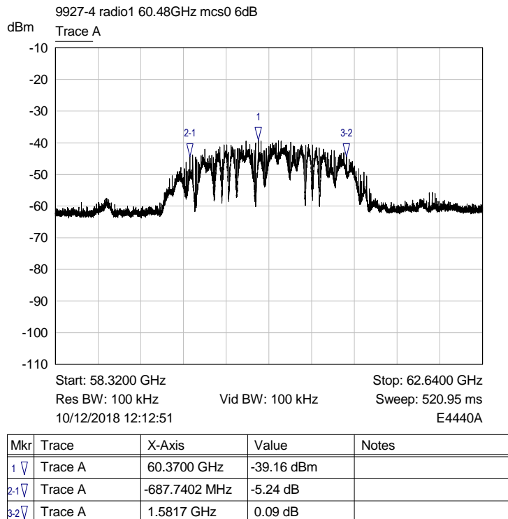
Plot for 6 dB Bandwidth (MHz) Nominal Temp & Volts
