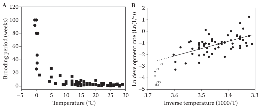
Figure 8 Brooding period and development rates of brooding marine gastropod snails at ambient temperatures for tropical to polar species. (A) Time from brood initiation to release ( 1/\text{development rate} ). Circles denote Antarctic species whereas squares denote Arctic, temperate and tropical species. In most cases, release is of crawling juveniles, but for two Antarctic species, Torellia mirabilis and Marseniopsis mollis release is of veliger larvae, and development time to juvenile is approximately double that of brooding, per se (Peck et al. 2006a). Data for 68 gastropod species, nine of which live at temperatures around 0°C, and are the full development period to juvenile. (B) Arrhenius plot of Ln developmental rate to juvenile stage for brooding gastropod molluscs. Open circles denote species living at temperatures below 3°C and closed circles show data for species living above 3°C. Fitted line is for temperate and tropical species (brooding rate (1/\text{weeks}) = 20.37 - 6.25 \text{ } 1000/T ; r^2 = 0.36 , F = 32.4 , 58 d.f., P < 0.001 ). (Figure from Peck, L.S. 2016. Trends in Ecology and Evolution 31 , 13–26.)
