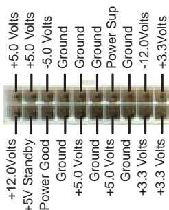
P2L97 ATX Power Connector
