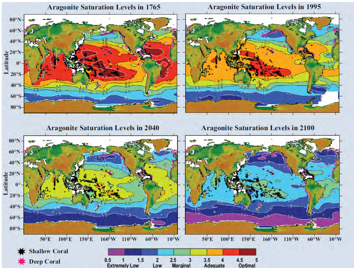
Figure 7. Estimated aragonite saturation states of the surface ocean for the years 1765, 1995, 2040, and 2100 (Feely et al. , submitted), based on the modeling results of Orr et al. (2005) and a Business-As-Usual CO 2 emissions scenario. The distributions of deep-sea coral banks are from Guinotte et al. (2006). Source: (Kleypas et al. 2006)
