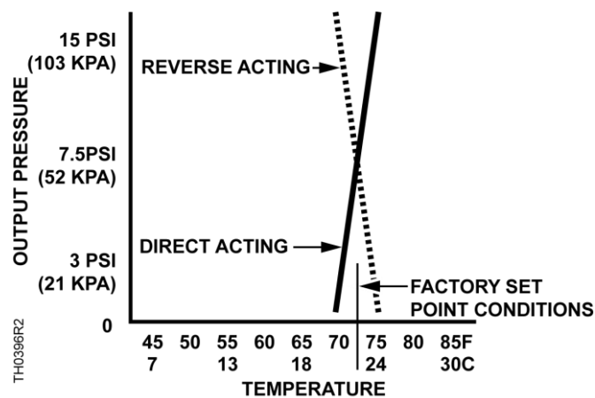
Figure 4. TH 192 HC Input/Output Characteristics.
