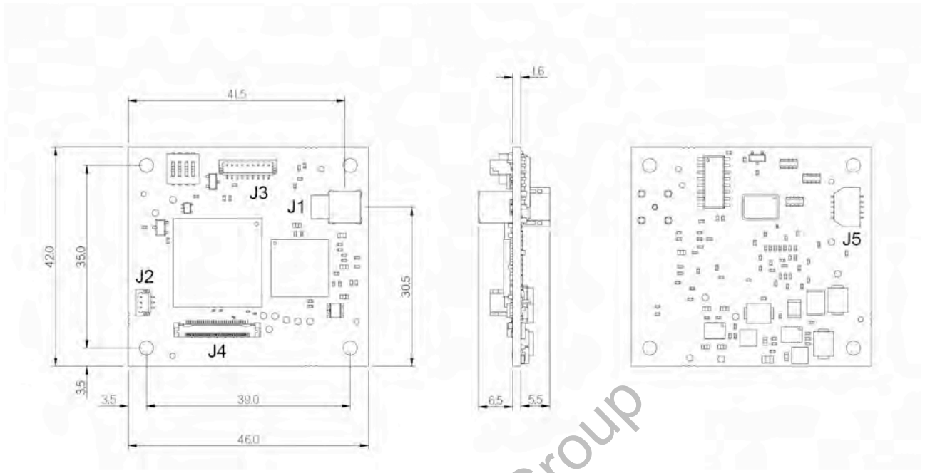
Figure 5: PCB mechanical details (top, side and bottom).
