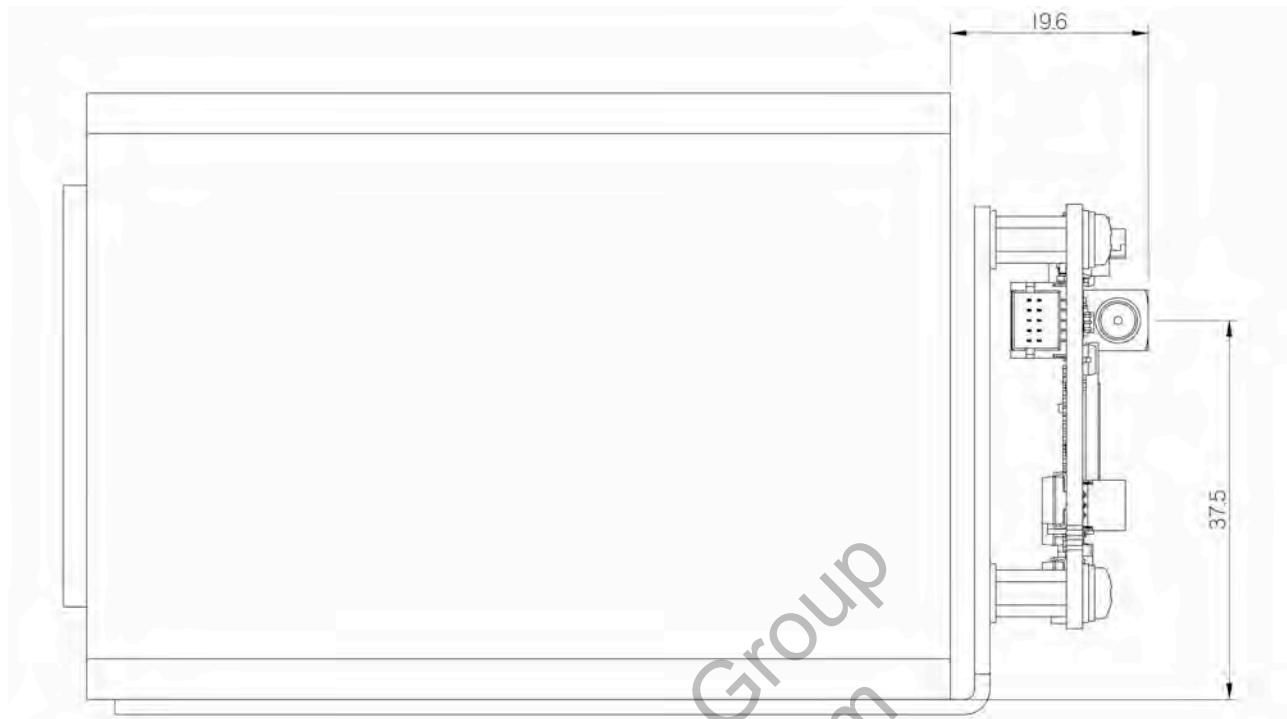
Figure 7: Module attached to EH6500 camera (side view).
