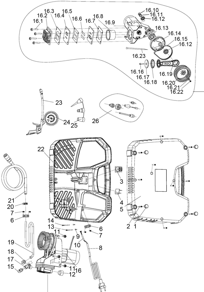
PUMP ASSEMBLY
