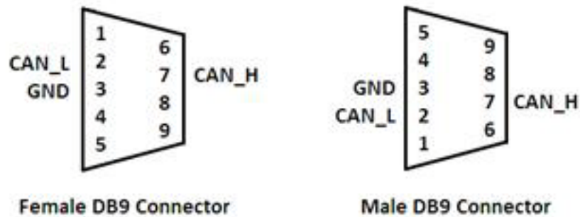
Figure 4.3 PCM-26D2CA DB-9 connector pin assignments
