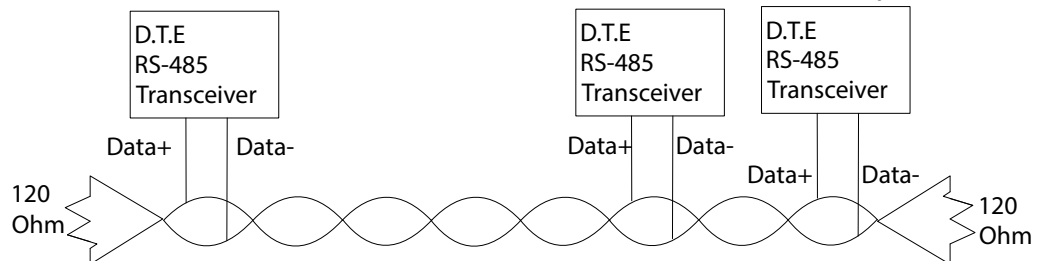
Figure 3.1 RS-485 Wiring Topology
