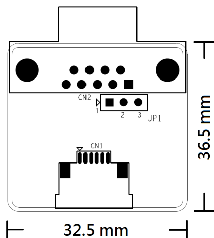
Figure 4.1 CAN-bus transceiver board silk screen
