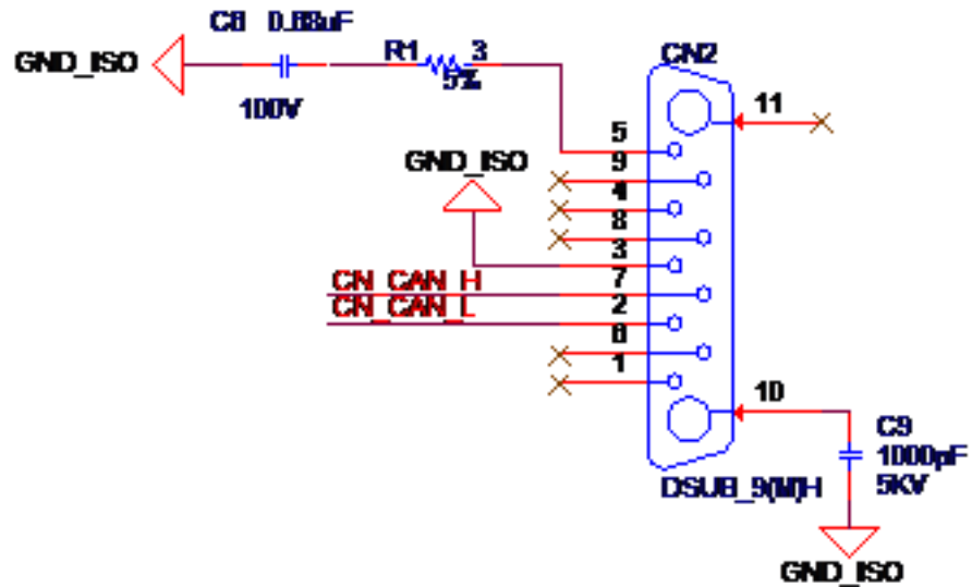
Figure 4.4 PCM-26D2CA DB-9 connector schematics
