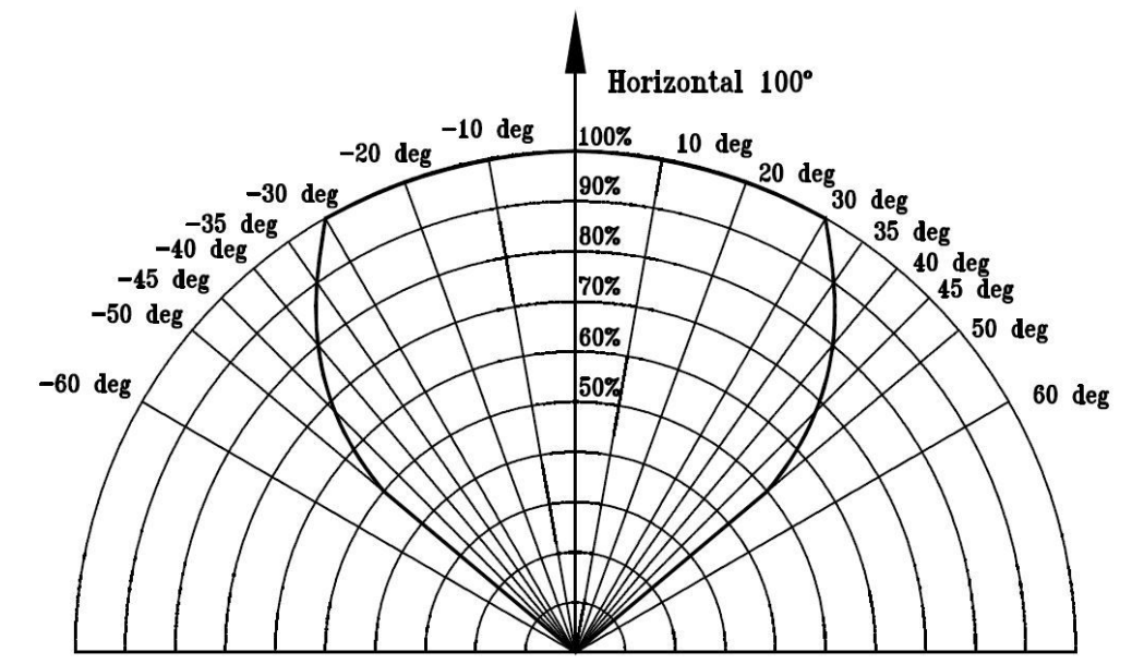
Figure 2-1: Horizontal field of view for Rosemount 975MR, 975UF, and 975UR
