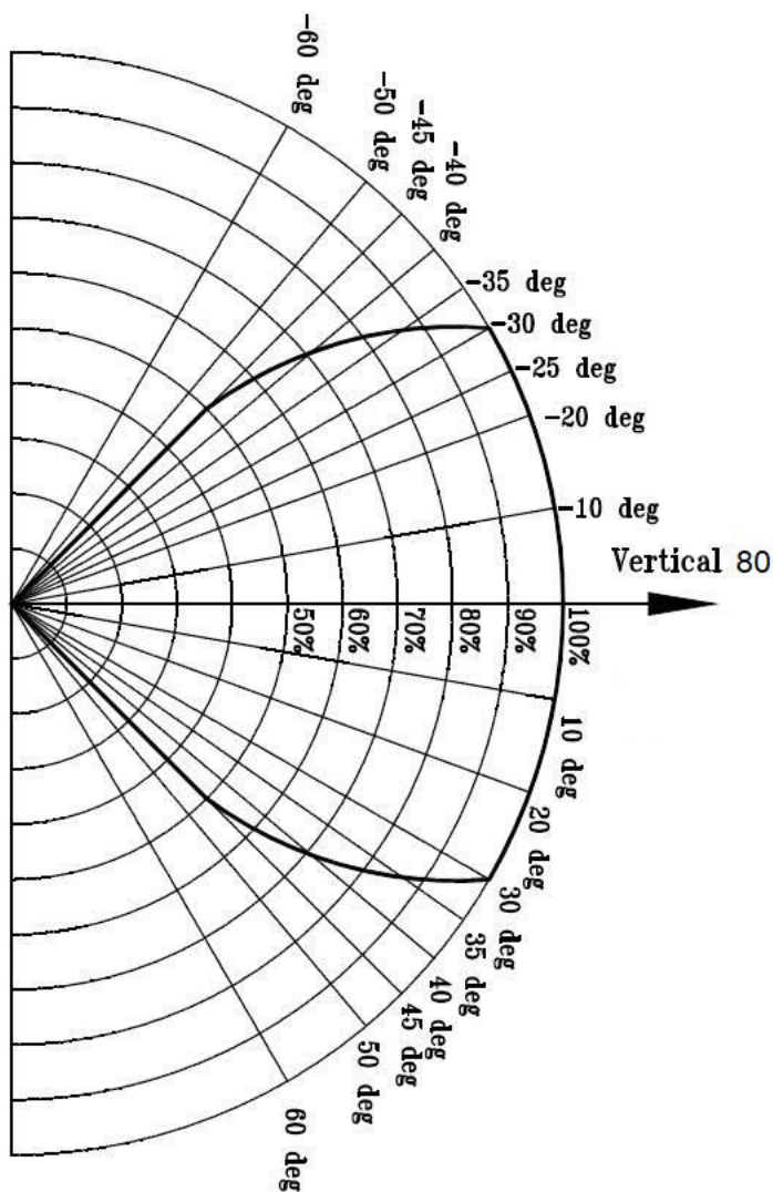
Figure 2-2: Vertical field of view for Rosemount 975MR, 975UF, and 975UR
