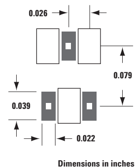
Figure 15. Recommended PCB Pad Layout for Avago's SC70 3L/SOT-323 Products.
