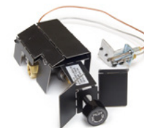
SPK-26(P) Low Profile Safety Pilot System
