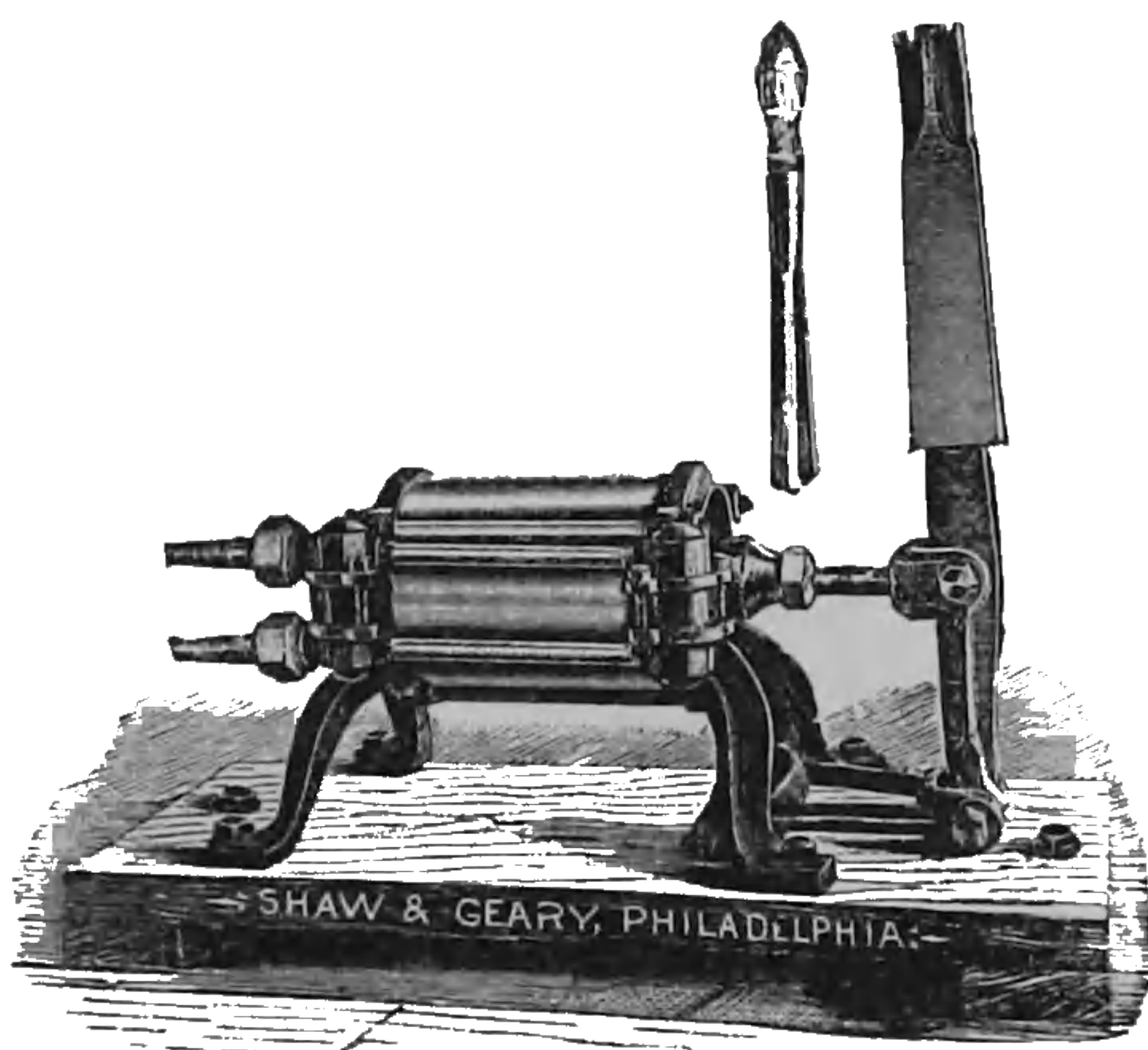
Double-acting air-pump.
