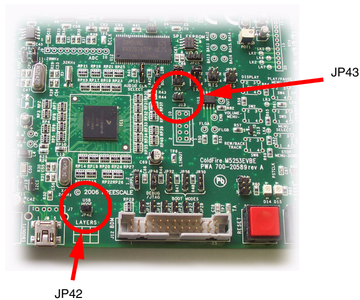
Figure 2. Location of JP42 and JP43 Jumper Blocks
