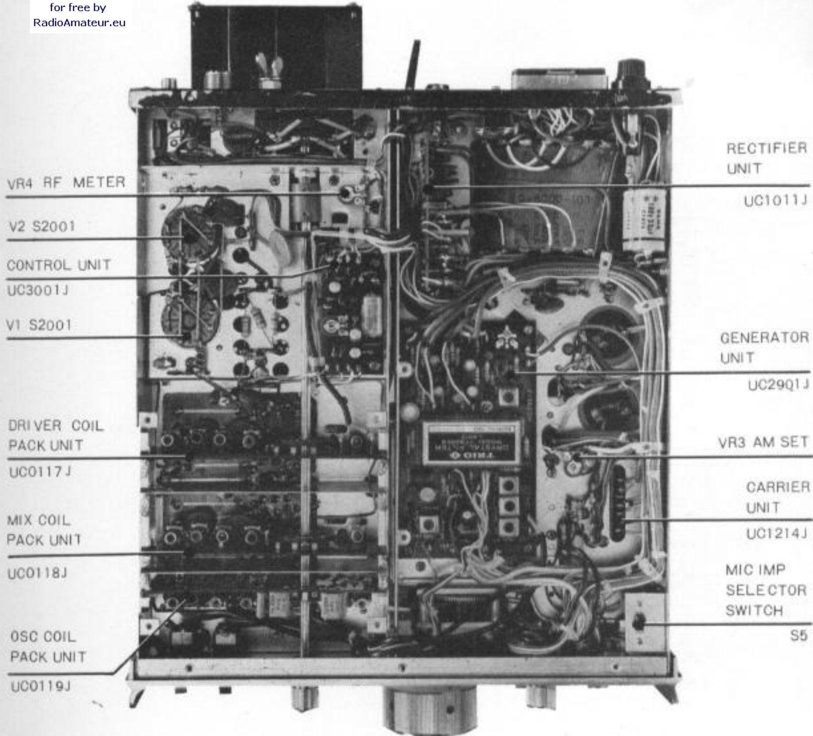
Figure 8 Bottom chassis view
