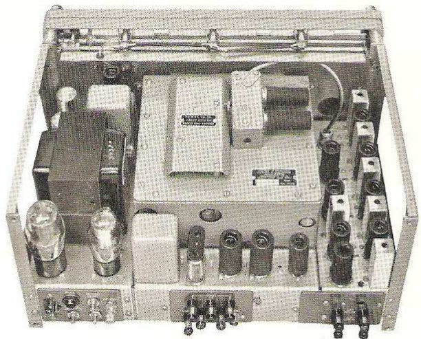
Rear view of the 770R receiver, illustrating the clean engineering lines and robust construction.
