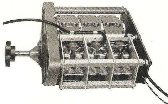
Tuning "heart" of the 770R receiver showing ganged capacitors, valve holders and, at the rear, part of the coil turret.
