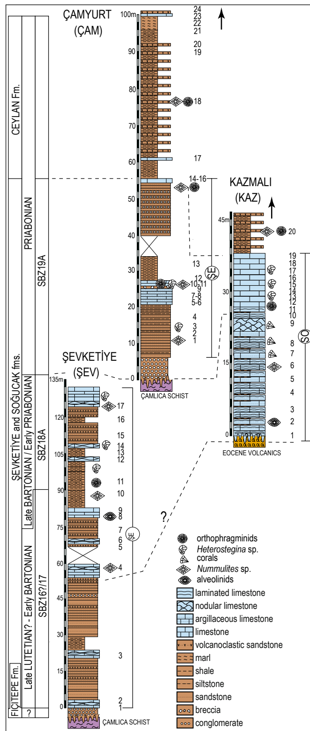
FIGURE 5. Lithostratigraphic columns of the Soğucak and Şevketiye fms. in the studied sections and their correlation. SBZ: Shallow Benthic Zones by Serra-Kiel et al. (1998), updated by Less and Özcan (2012). E: Şevketiye Fm., SO: Soğucak Fm.
