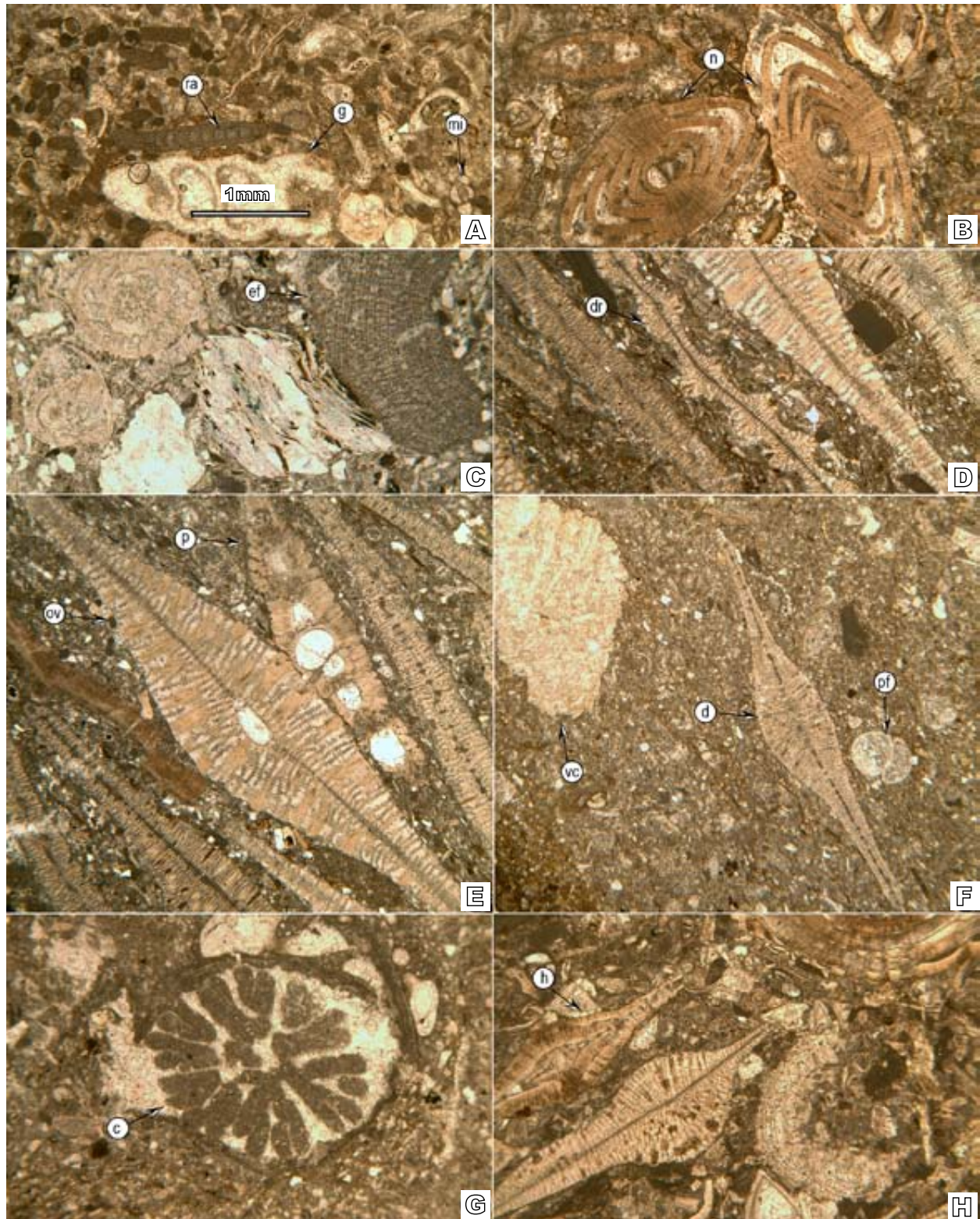
FIGURE 7. Thin-section microphotographs of the fossil associations from the Şevketiye (A–F) and Soğucak (G–H) fms. A) Red algae-gastropod packstone (ŞEV2) and B) nummulitid packstone (ŞEV4) in the lower part of the Şevketiye Section. C) Siltstone/sandstone level with encrusting foraminifera (ÇAM1), and D–E) orthoherminids and Pellatispira (ÇAM4) in the lower part of the Soğucak Fm. In the Çamyurt Section. F) Shale/siltstone facies with planktonic foraminifera, orthoherminids and volcanic fragments in the Çamyurt Section (ÇAM13). G) Corals encrusted by red algae in the lower part (KAZ8), and H) foraminiferal packstone (KAZ16) in upper part of the Soğucak Fm. in the Kazmalı Section. Abbreviations: c, corals; d, Discocyclina sp.; dr, Discocyclina radians ; ef, encrusting foraminifera; g, gastropods; h, Heterostegina ; mi, miliolids; n, Nummulites ; ov, Orbitoclypeus varians ; p, Pellatispira madaraszi ; pf, planktonic foraminifera; ra, red algae; vc, volcanic fragments.
