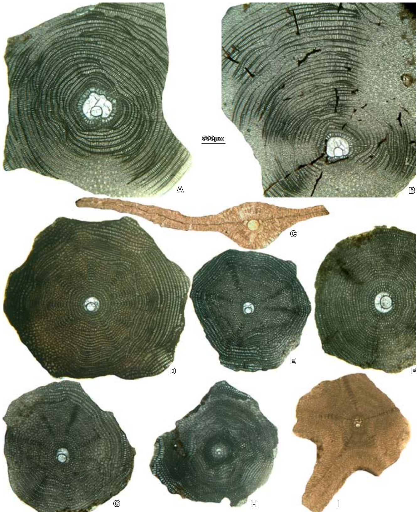
FIGURE 14. Orthophragminids from the Şevketiye (A–C, E–I), and Soğucak (D) fms. in Çamyurt and Kazmalı sections (SBZ19). A–C) Discocyclina pratti pratti . A) sample ÇAM14-37, B) sample ÇAM14-12, C) sample ÇAM17-1; D) Orbitoclypeus varians scalaris , sample KAZ11-29; E–G) O. varians varians . E) sample ÇAM14-28, F) sample ÇAM14-2, G) sample ÇAM14-26; H) Nemkovella daguini , sample ÇAM14-25; I) Asterocyclina stellata , sample ÇAM10-3.
