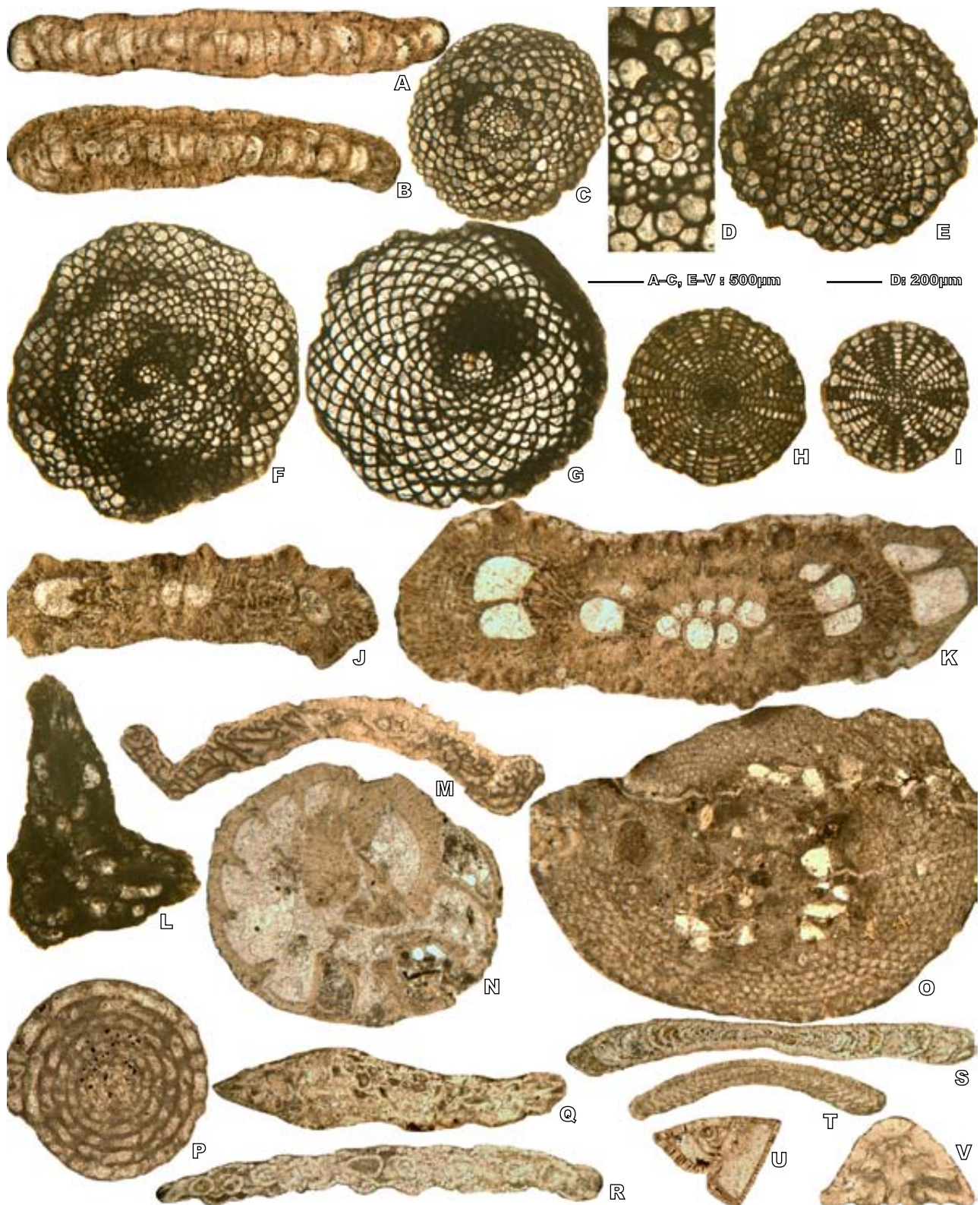
FIGURE 16. Foraminifera and other fossils groups in the Şevketiye (A–L, N–P, S–T), and Soğucak (M, Q–R, U–V) fms. A–G) Linderina sp. A–B) Sample ŞEV10, C–G) sample ŞEV11. H–I) Sphaerogypsina globula . H) Sample ŞEV11, I) sample ŞEV10. J–K) Pellatispira madarazsi . J) Sample ÇAM4, K) sample ÇAM6. L) Silvestriella tetraedra . Sample ŞEV17. M) Fabiania cassis . Sample KAZ15. N) Gyroidinella magna . Sample ÇAM1. O) Orbitolites sp. Sample ŞEV3. P) Praebullalveolina afyonica . Sample KAZ16. Q–R) encrusting foraminifera. Q) Sample KAZ14, R) sample ÇAM16. S–T) Eoannularia eocenica . S) Sample ÇAM8, T) sample ÇAM16. U–V) Rotalids. Sample KAZ12.
