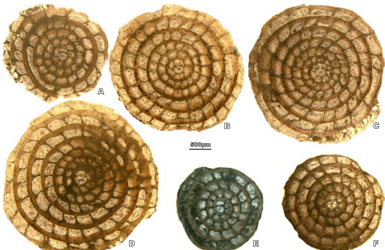
FIGURE 13. Reticulate Nummulites from the Şevketiye (A–E) and Soğucak (F) fms. in Çamyurt and Kazmalı sections (SBZ19A, 19A/20, respectively). A–F: Nummulites fabianii . A) Sample ÇAM3-2, B) sample ÇAM3-3, C) sample ÇAM3-4, D) sample ÇAM3-8, E) sample ÇAM14-21, F) sample KAZ11-9.
