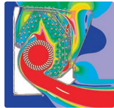
Fast ← → Slow Colours in the figure show the air speed.
