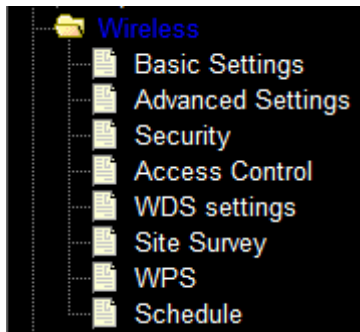
Figure 4-15 Wireless menu
