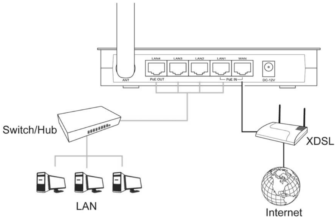
Figure 2-1 Hardware Installation of the WLAN 11N AP
