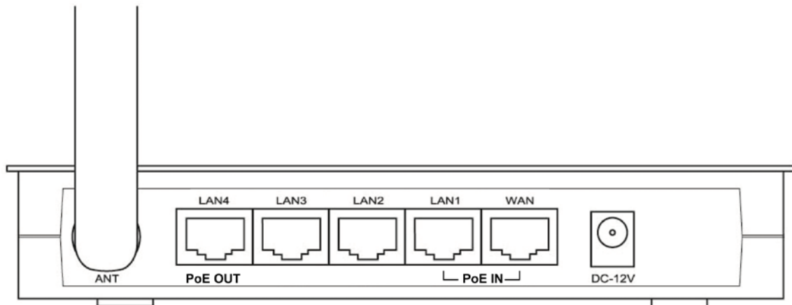
Figure 1-2 Rear Panel sketch
