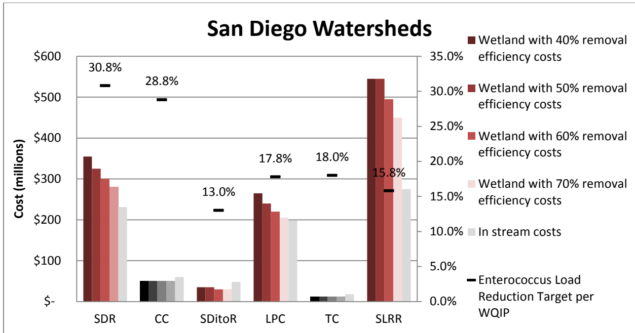
Figure E-1. Results of Sensitivity Analysis for San Diego County Watersheds on Total Costs for Off-Line Wetlands for Various Wetland FIB Reduction Efficiencies
