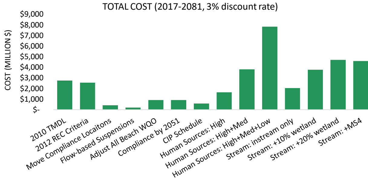
Figure 38: The total cost of meeting the required load reduction through the implementation and maintenance of BMPs is highest for the Human Sources: High+Med+Low scenario and lowest for the Flow-based Suspensions scenario.
