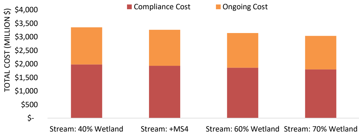
Figure 46: Bars indicate alternatives to the Stream: + MS4 scenario with varying wetland removal efficiency and varying the number of projects implemented to achieve the required load reduction. Varying the number of projects varies the scenario cost. Difference in bar height indicates the sensitivity of total scenario cost to changing these two inputs.
