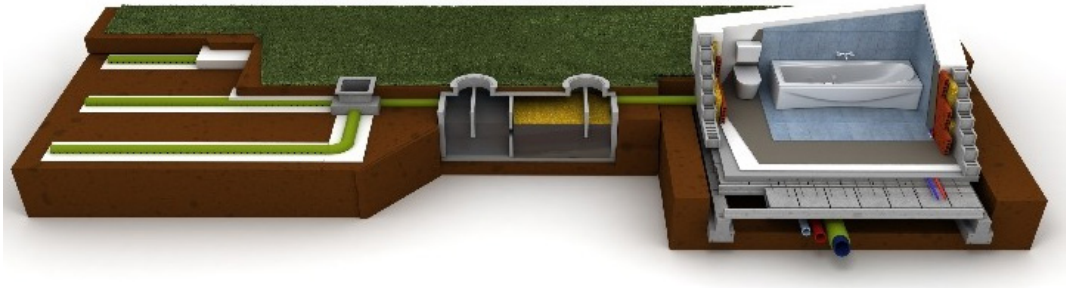
Figure 6-2. Typical Septic System Layout (DEH 2017)
