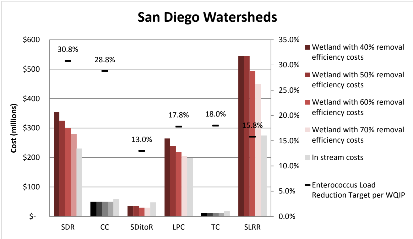
Figure 1. San Diego County Wetlands Cost Comparison
