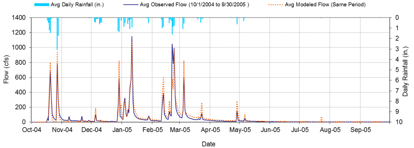
Figure 9. Example hydrologic (flow) calibration. Mean daily flow: Model Outlet 4050181 vs. USGS 11022480 San Diego R at Mast Rd near Santee CA
