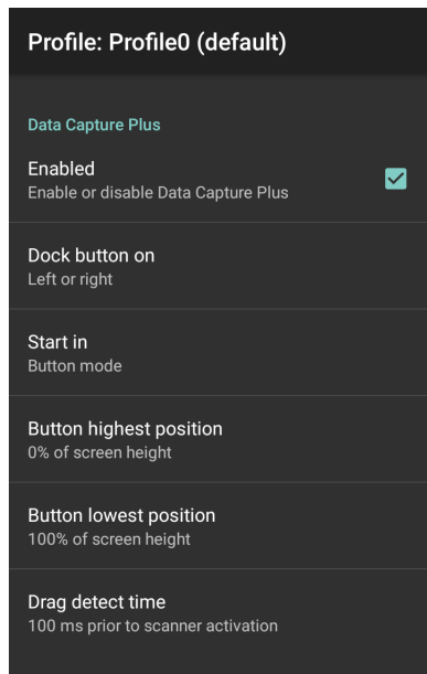
Figure 86 Data Capture Panel Settings
