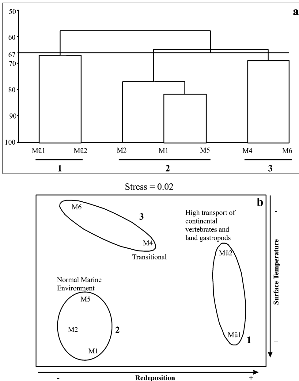
Fig. 4 a-b: (a) hierarchical agglomerative clustering based on the Bray-Curtis Similarity and (b) non-metric Multidimensional Scaling (nMDS) plot of planktonic foraminifera from the Mühlbach Section.
