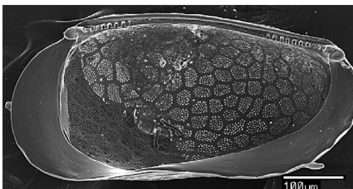
5: Right valve interior showing hinge and pore clusters (SEM). 1-5: from MADDOCKS (2006).
